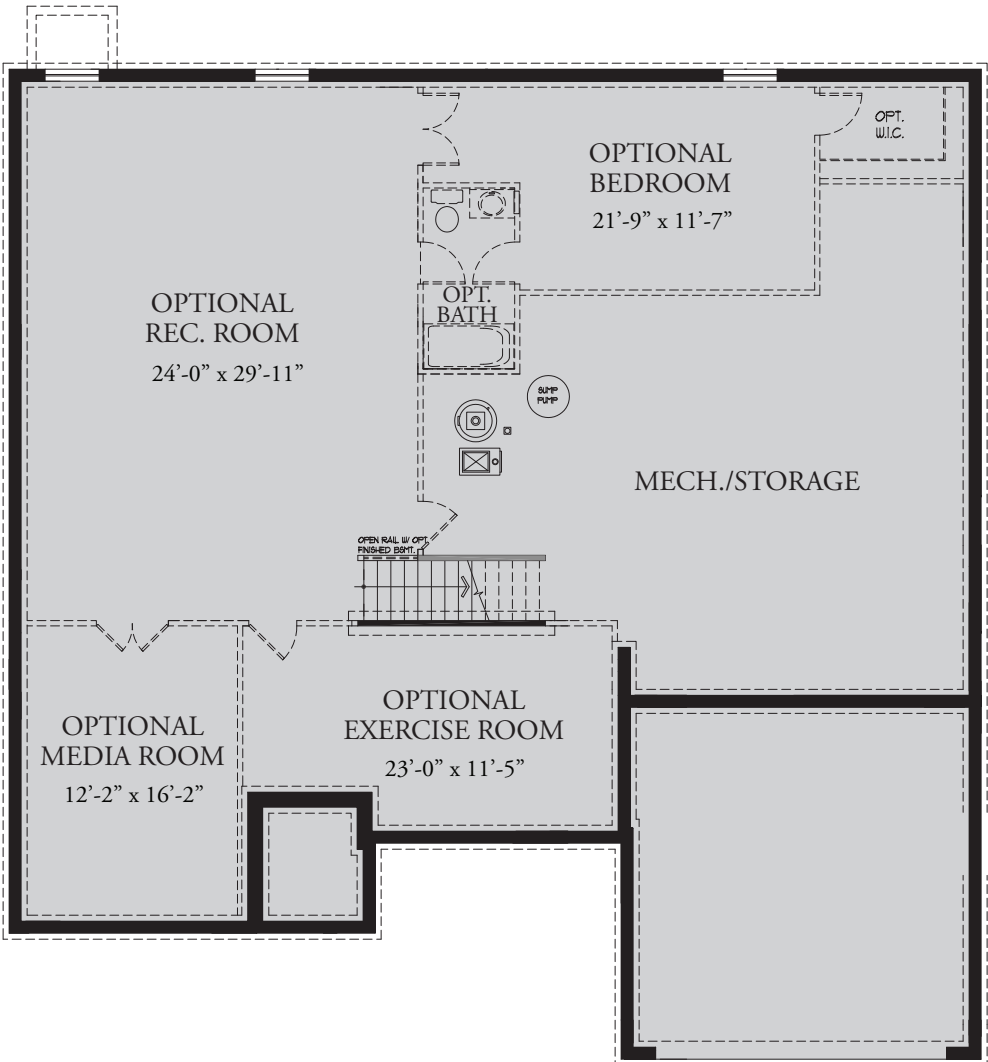
PARTIAL FOUNDATION PLAN W/ OPT. SLIDING DOOR @ WALK-OUT COND.
