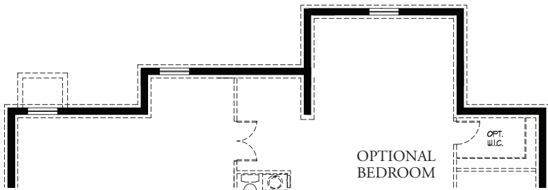
PARTIAL FOUNDATION PLAN W/ OPT. 4' EXTENDED FAMILY ROOM AND MORNING ROOM
