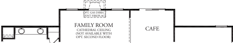
PARTIAL FIRST FLOOR PLAN W/ 4' EXTENDED FAMILY ROOM & EXTENDED CAFE
