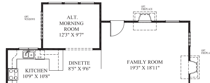
PARTIAL FIRST FLOOR PLAN W/ OPT. ALT. MORNING ROOM & OPT. 6 FT. EXTENDED FAMILY ROOM
