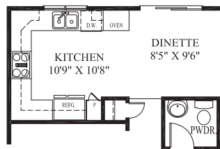
PARTIAL FIRST FLOOR PLAN W/ OPT. GOURMET KITCHEN
