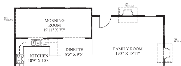
PARTIAL FIRST FLOOR PLAN W/ OPT. MORNING ROOM & OPT. 6 FT. EXTENDED FAMILY ROOM
