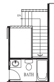
PARTIAL SECOND FLOOR PLAN W/ OPT. BATH ABOVE FOYER
