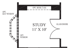
PARTIAL FIRST FLOOR PLAN W/ OPT. STUDY
